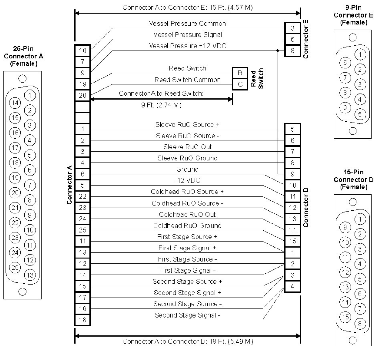
Illustration 6-17: Magnet Monitor Cable B (Run 830): 2222797
